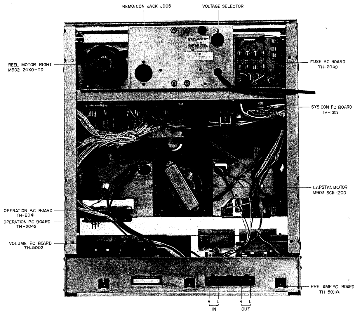
Fig. 3 Rear View
