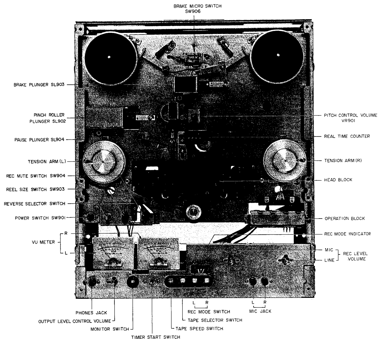
Fig. 2 Front View
