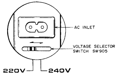
Fig. 1 Voltage Conversion (CEE, UK Model)
