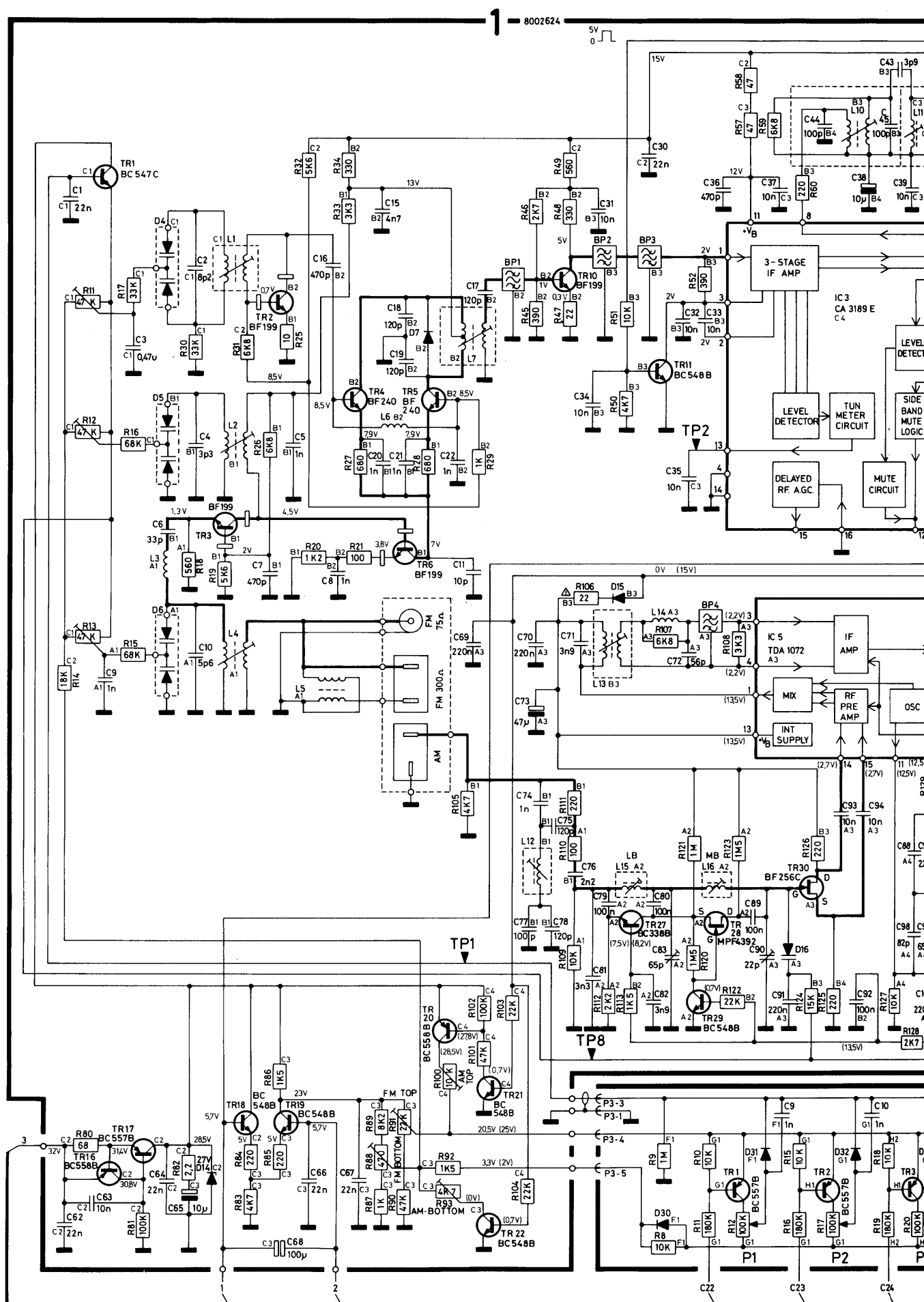
DIAGRAM A, type 2912/17 Before serial no. 2930001
